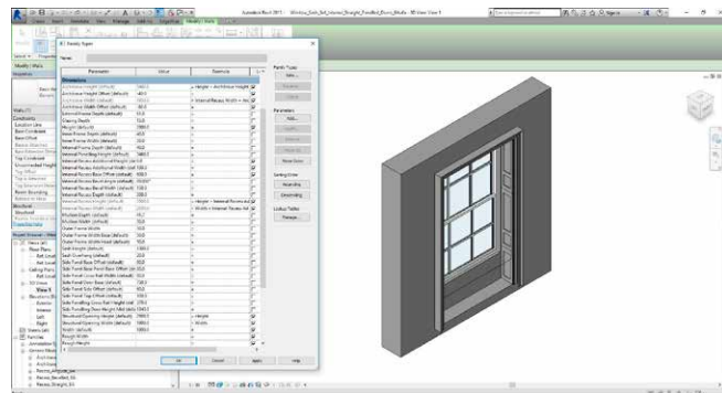
Figure CS4.4 The family type parameters that allow the identification of individual parts of each window.
